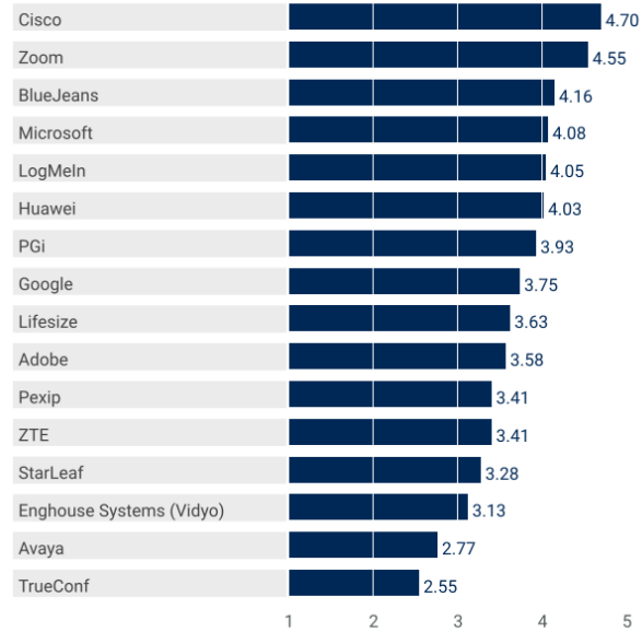
Figure 4. Vendors' Product Scores for Webinars Use Case
