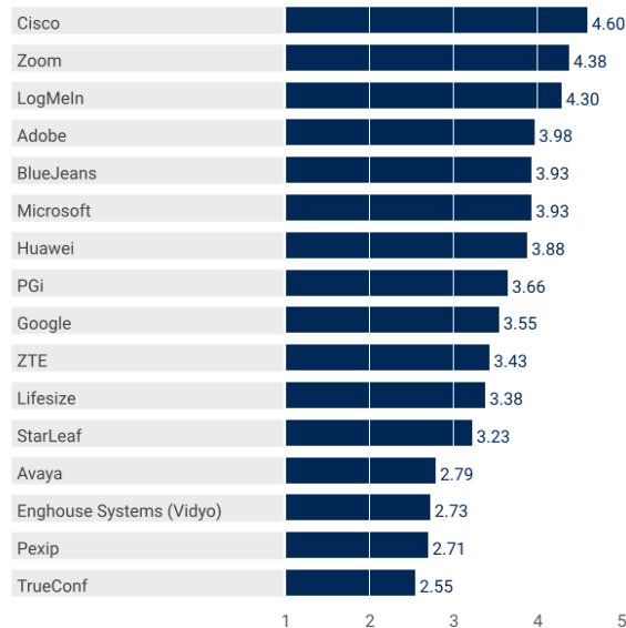
Figure 2. Vendors' Product Scores for Learning and Training Use Case
